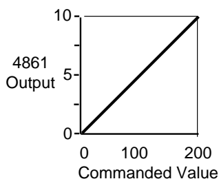
Example for a 0 to 200 volt supply with M = .05 , B = 0
