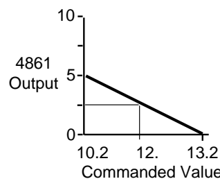
Example for a 12V \pm 10\% supply with M = -2.083 and B = 27.5
