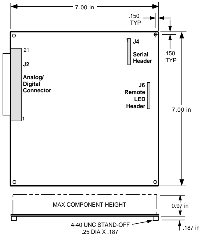
Figure 2 2361A OEM Board Dimensions
