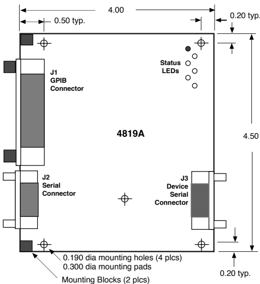
4819A Outline Dimensions
