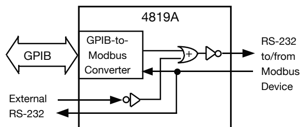
Figure 1 4819A Data Paths
