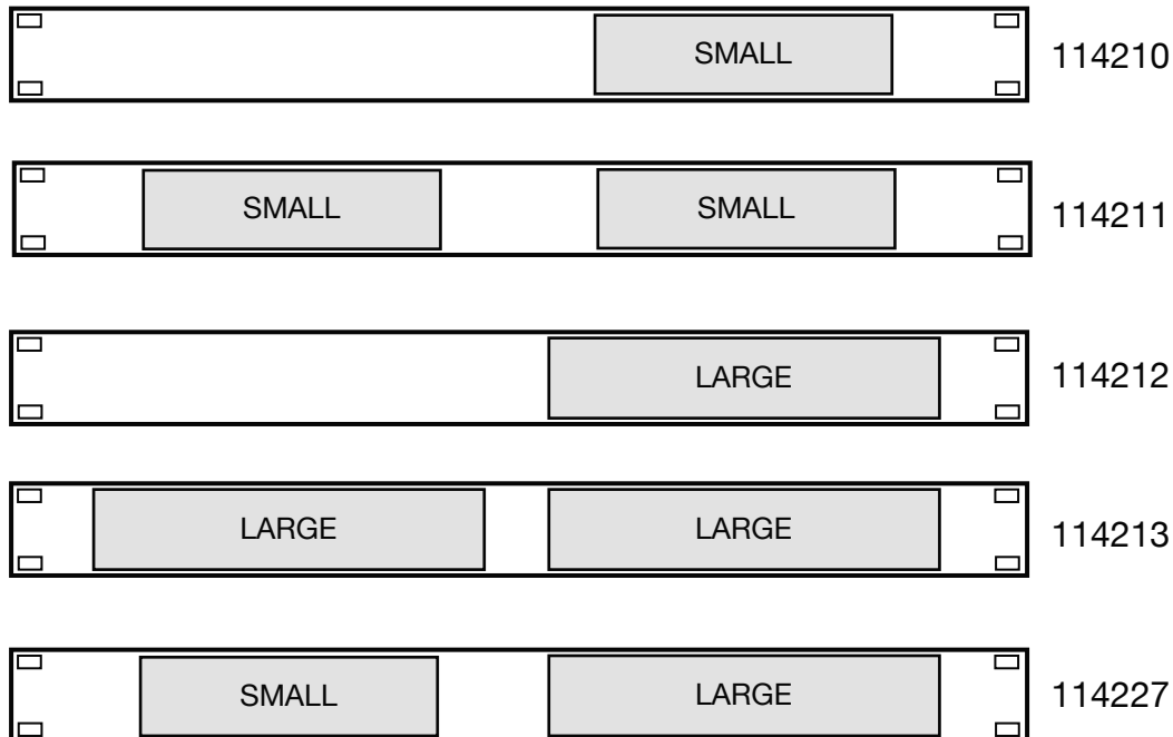
Minibox Rack Mounting Kits with Module Locations
