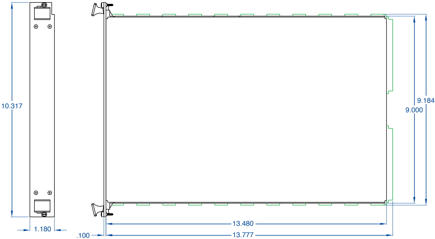
Figure 1 C-Size ITC style VXI Shield Kit
